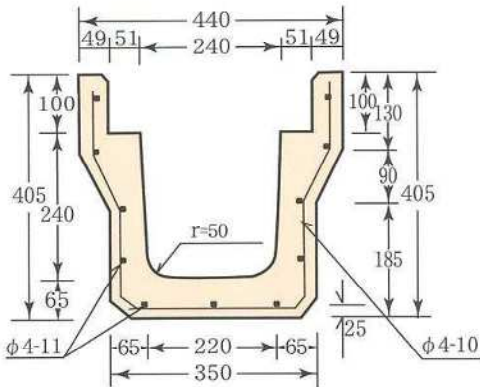
PU3型-240 ( \ell = 1,000 )
